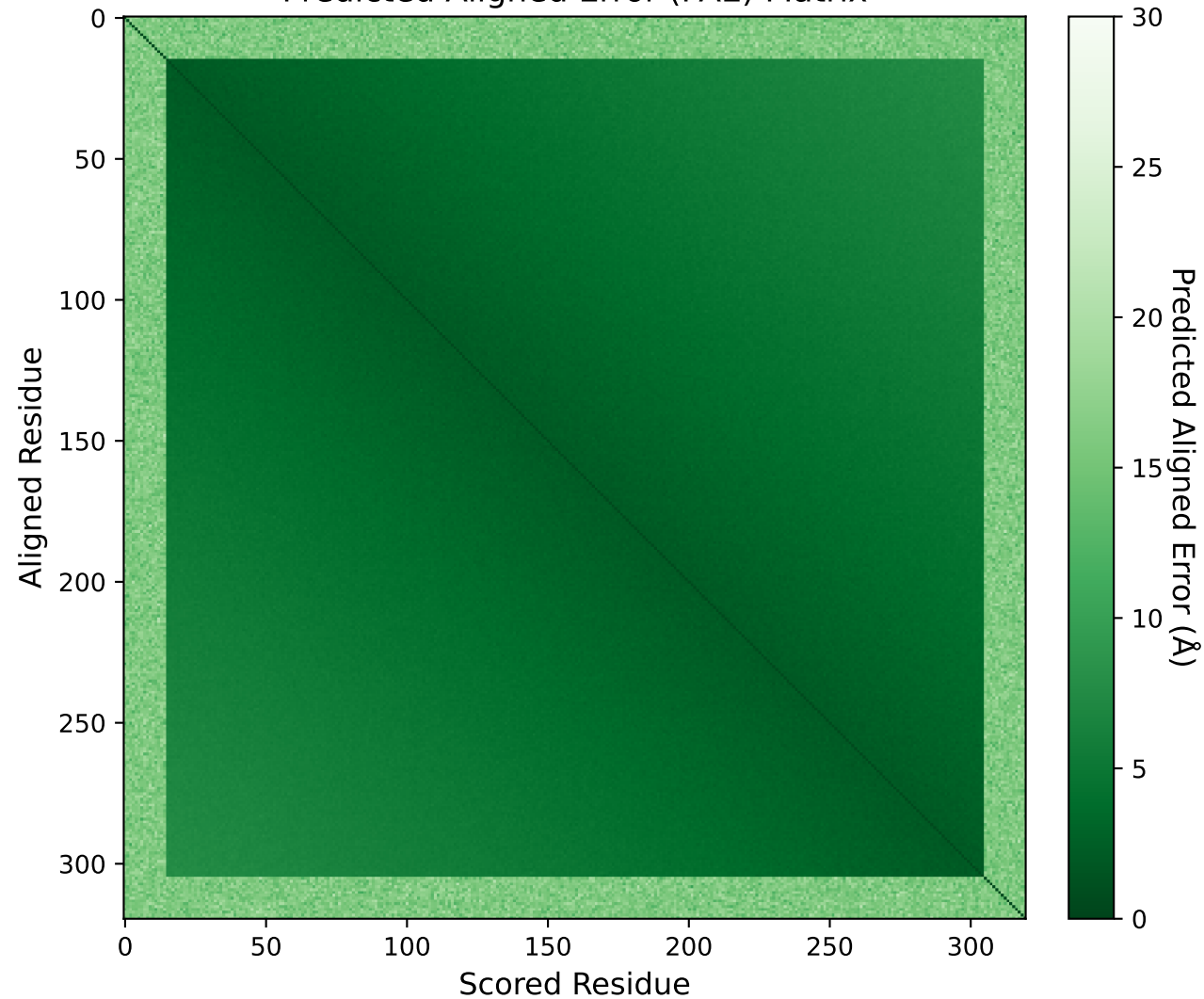
Predicted Aligned Error (PAE) Matrix
