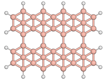
\beta_{12} B 44 H 16 (metallic, E_F \approx -6.54 eV)
