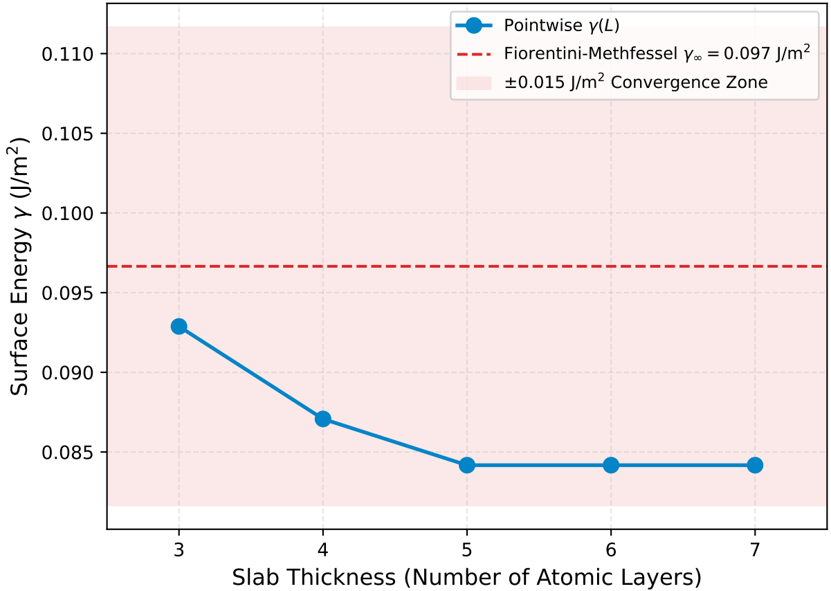
Pt(111) (p(2x2) 4-atom/layer slab) — Surface Energy Convergence ( \gamma = 0.084 \text{ J/m}^2 )
