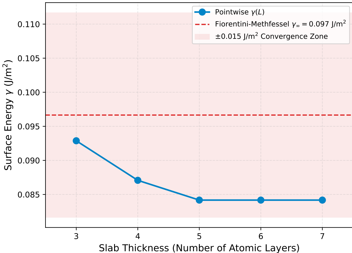
Pt(111) — Surface Energy Convergence ( \gamma = 0.084 \text{ J/m}^2 )
