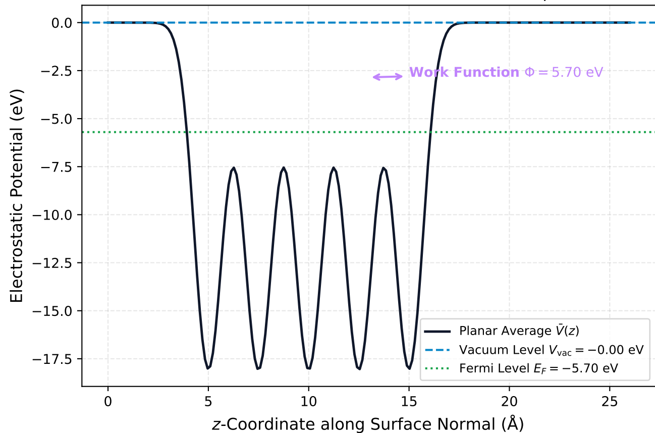
Planar Electrostatic Potential Profile — Vacuum Gap = 16.0 Å
