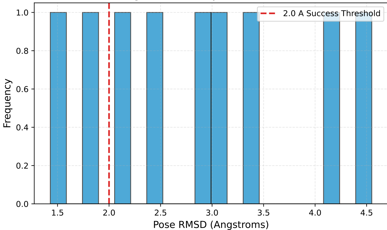
Redocking Pose Accuracy (Best RMSD = 1.43 Å)
