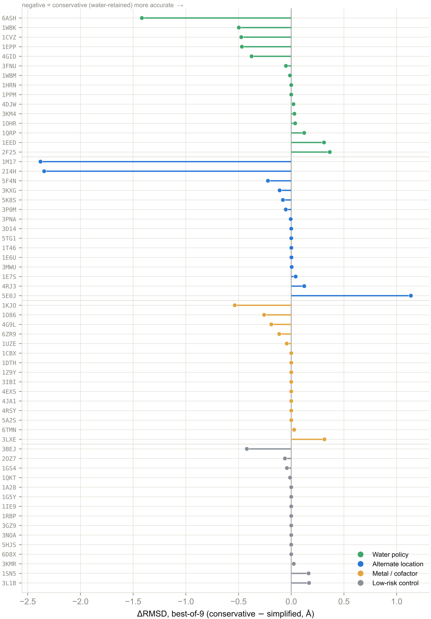
Per-case water-policy effect on redocking accuracy, all 60 cases
