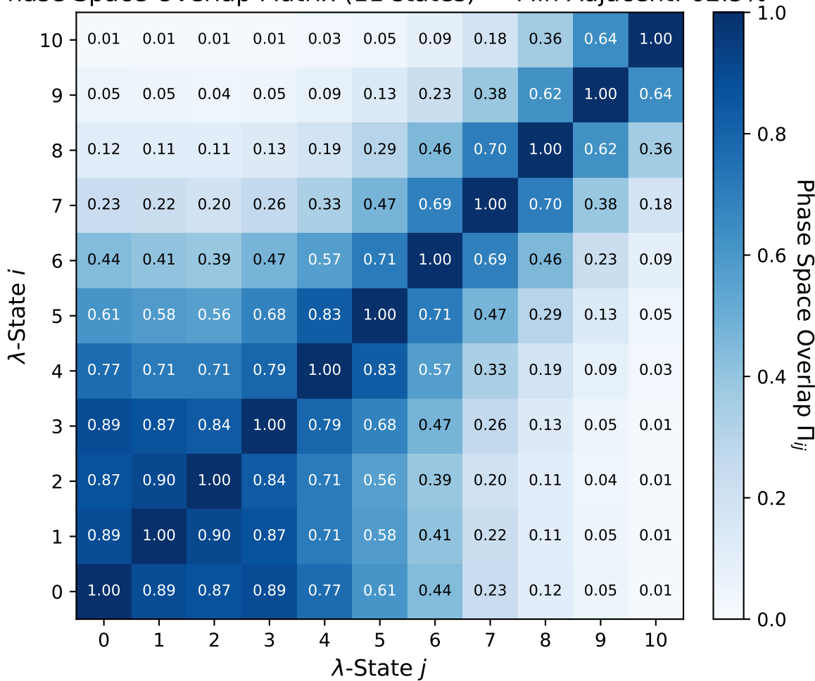
Phase Space Overlap Matrix (11 states) — Min Adjacent: 62.5%
