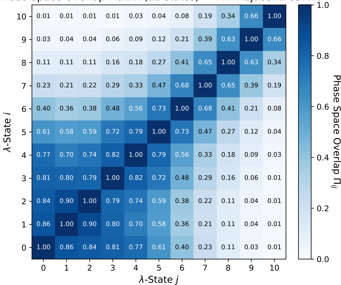
Phase Space Overlap Matrix (11 states) — Min Adjacent: 63.4%
