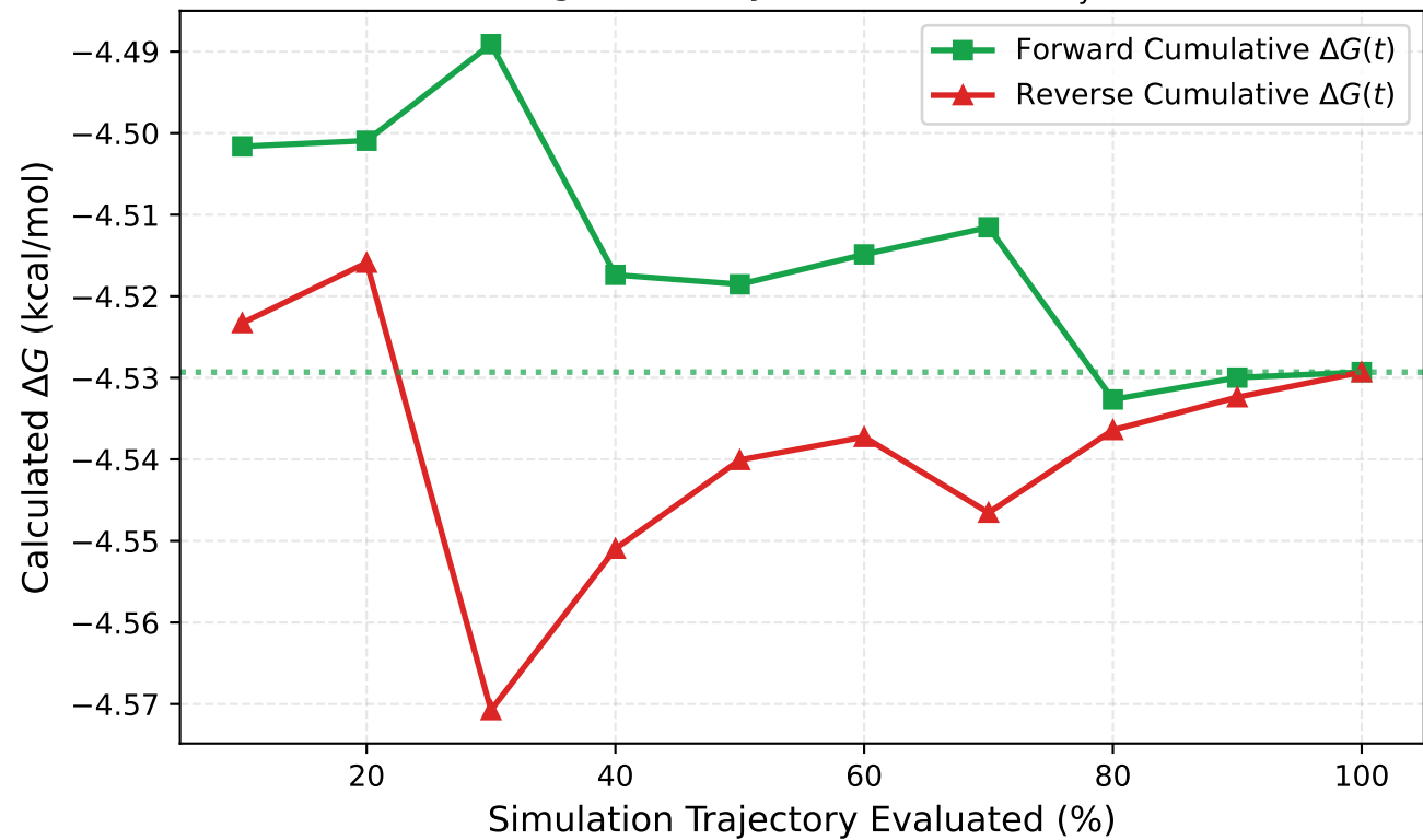
Time-Series Convergence & Hysteresis — \Delta\Delta G_{\text{hyst}} = 0.00 kcal/mol
