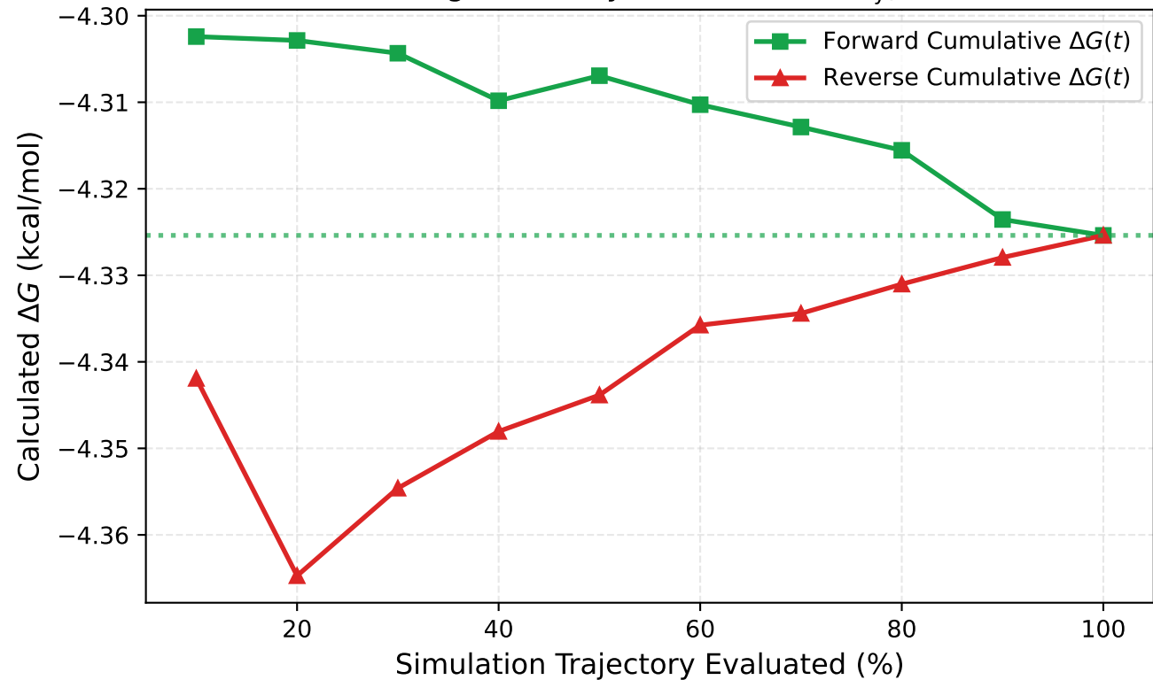
Time-Series Convergence & Hysteresis — \Delta\Delta G_{\text{hyst}} = 0.04 kcal/mol
