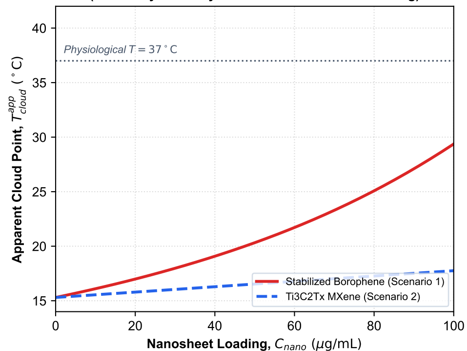
(a) True Apparent Cloud-Point Shift ( T_{cloud}^{app} ) (Thermodynamically Solved via Brent's Root Finding)
