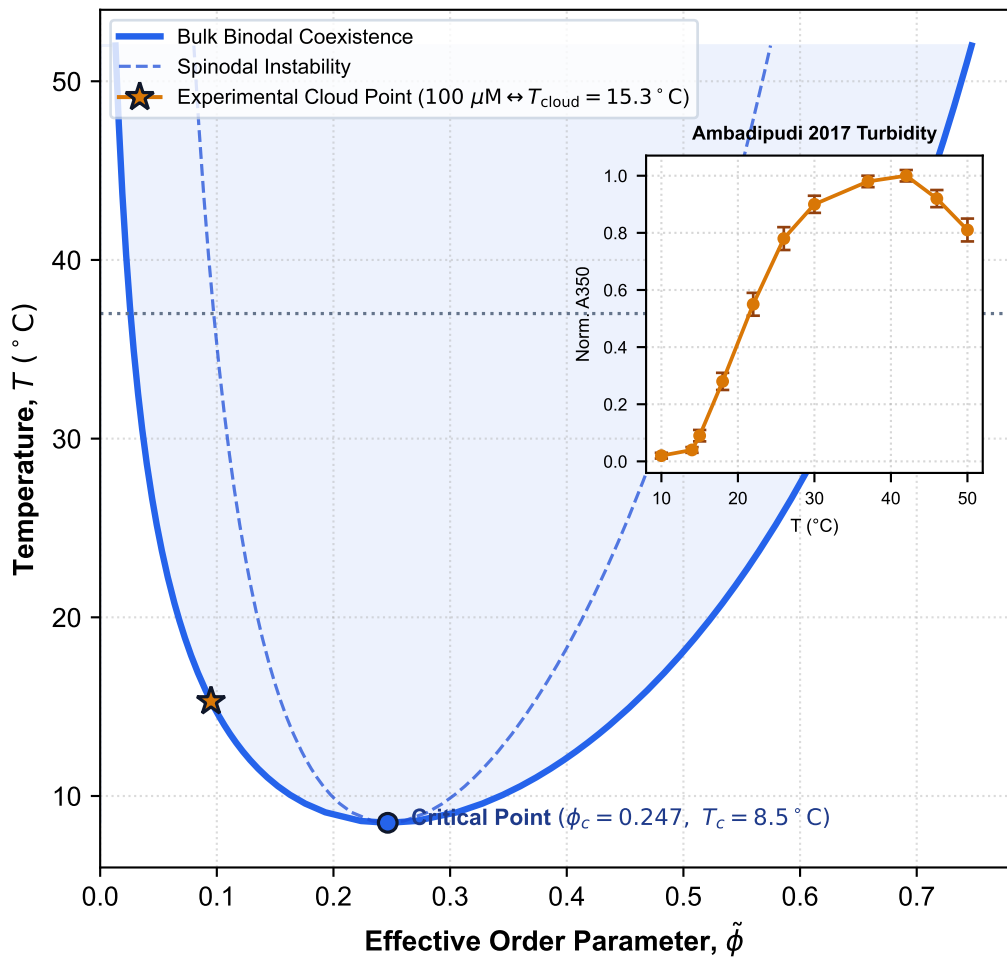
(a) Tau K18 Bulk LCST Phase Coexistence (Parameterized to Onset at 15.0 – 15.3 °C, Ambadipudi et al. 2017)
