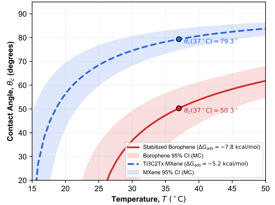
(b) Condensate Wetting Angle \theta_c(T) (Young's Eq. with Monte Carlo 95% CI)
