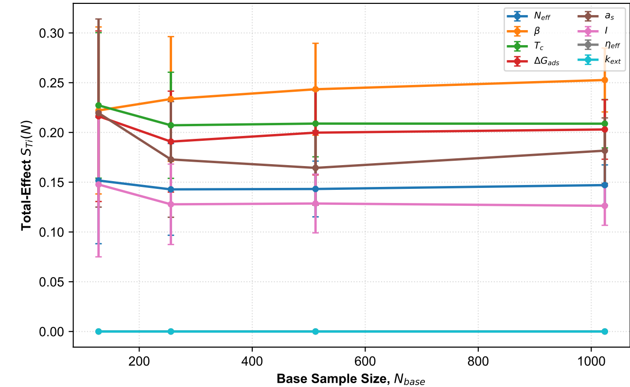
(c) Block Sensitivity Trajectories: T_{cloud}^{app} Indices
