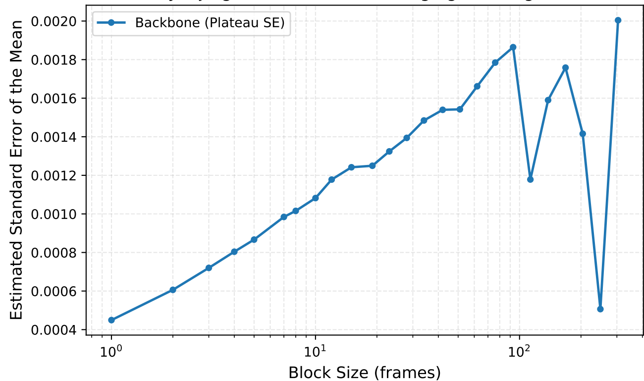
Flyvbjerg-Petersen Block Averaging Convergence
