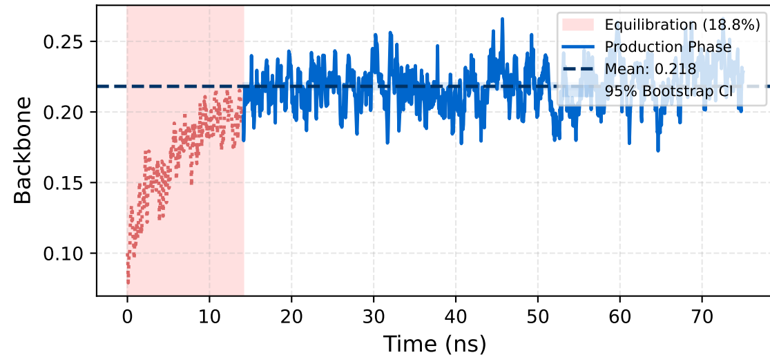
Backbone Trajectory & Equilibration Cutoff ( t_{eq} = 14.11 ns)
