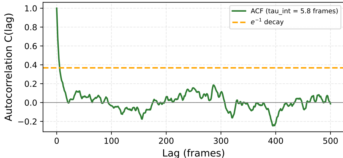
Backbone Autocorrelation ( N_{eff} = 105 )
