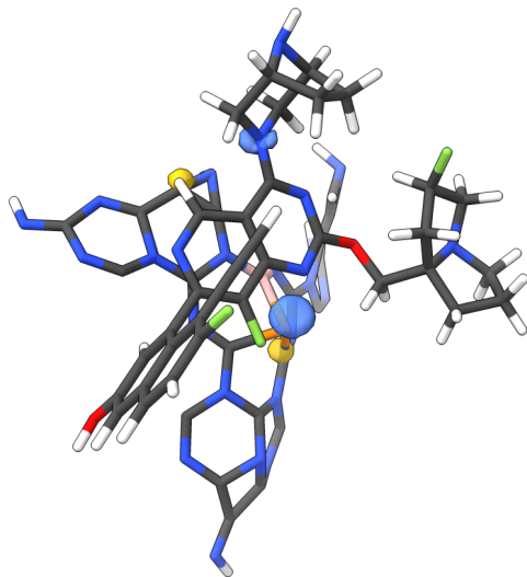
(a) KRAS-G12D / g-C 3 N 4
