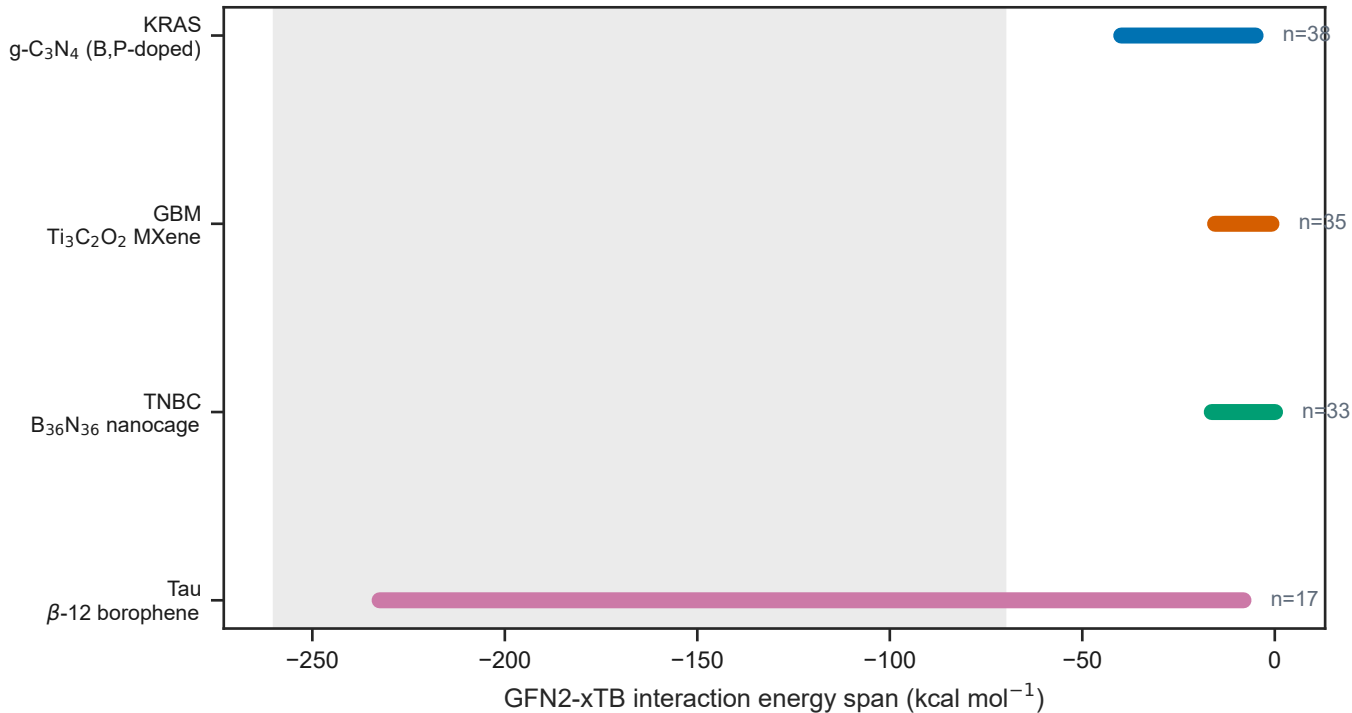
Figure 2. Interaction-energy regimes across the four 2D-carrier case studies
