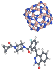
b Olaparib (physisorption)
