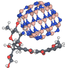
c Epirubicin (physisorption)
