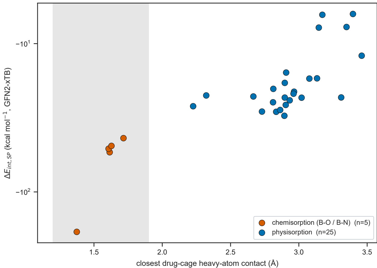
Figure 11. Adsorption landscape of 30 anti-TNBC drugs on pristine B 36 N 36
