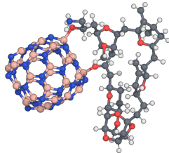
d Eribulin (chemisorption)
