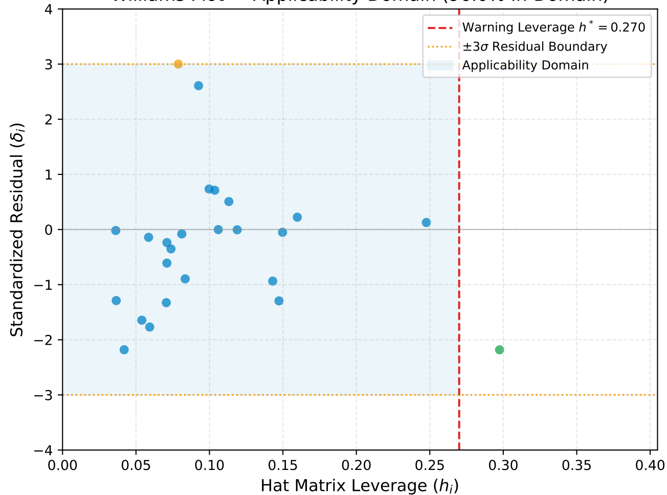
Williams Plot — Applicability Domain (96.0% In-Domain)
