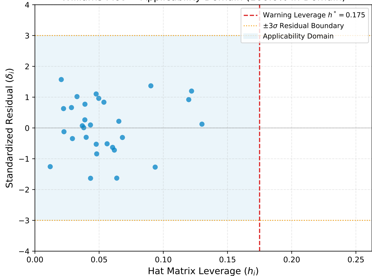
Williams Plot — Applicability Domain (100.0% In-Domain)
