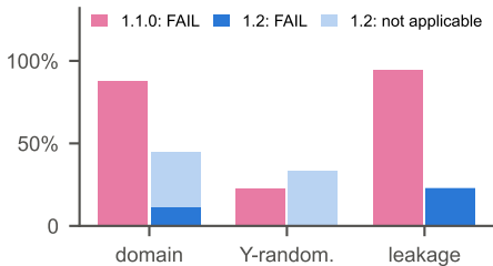
Verdicts on 180 real models
