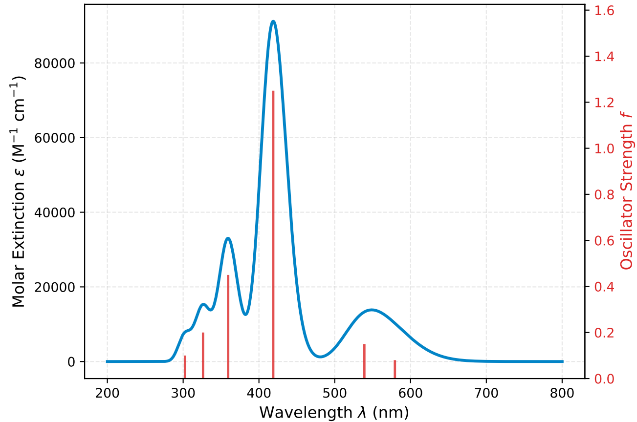
TD-DFT UV-Vis Spectrum — \lambda_{\text{max}} = 418.4 \text{ nm}
