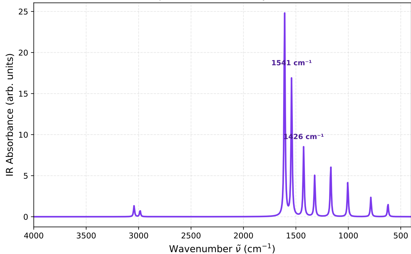
IR Vibrational Spectrum — Scaled by 0.9570 (wB97X-D)
