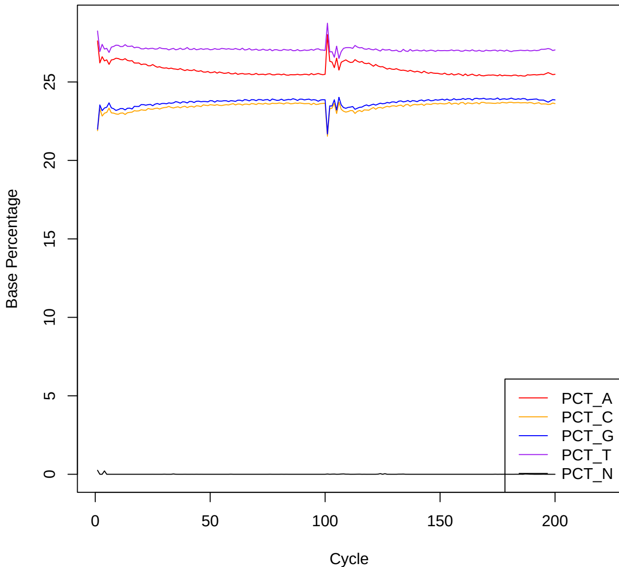
Base Distribution by Cycle in file normal_marked.bam (normal)
