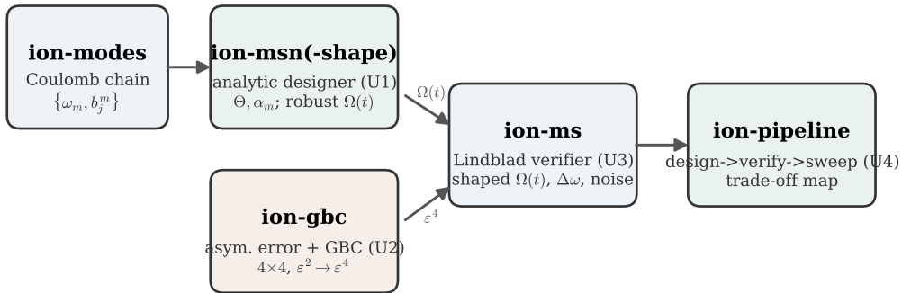
Fig. 1 — toolchain: analytic design ( O(M) ) \rightarrow open-system verify \rightarrow noise sweep
