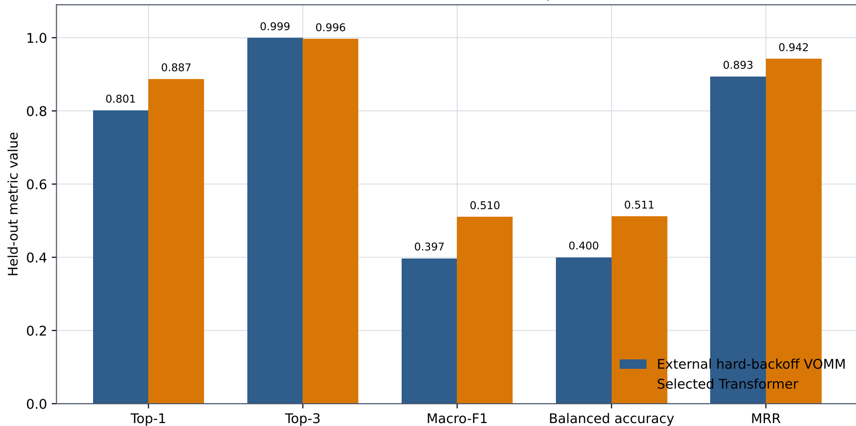
Overall held-out model comparison
