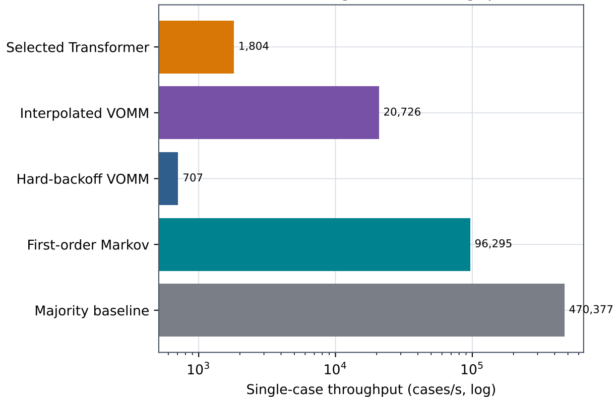
Real-time single-case throughput
