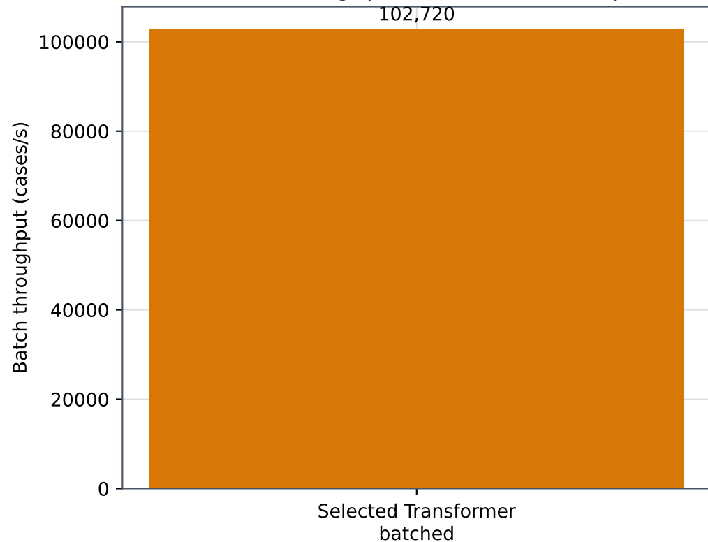
Offline batch throughput (not real-time equivalent)
