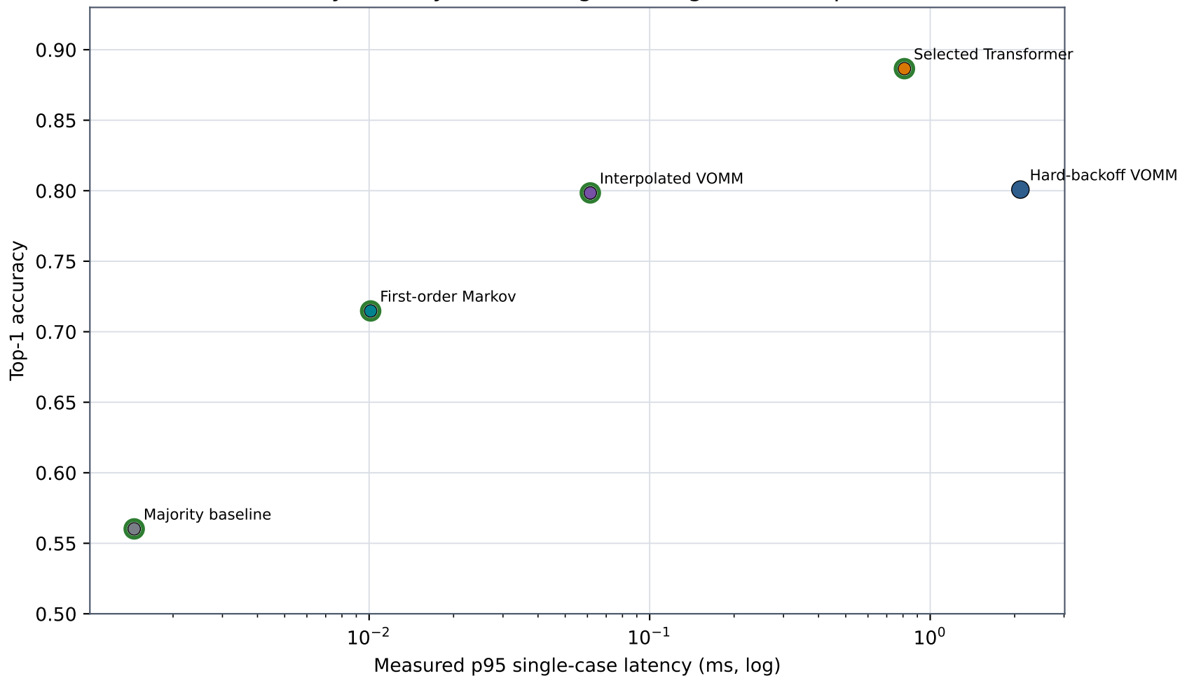
Accuracy-latency trade-off (green rings: Pareto-optimal)
