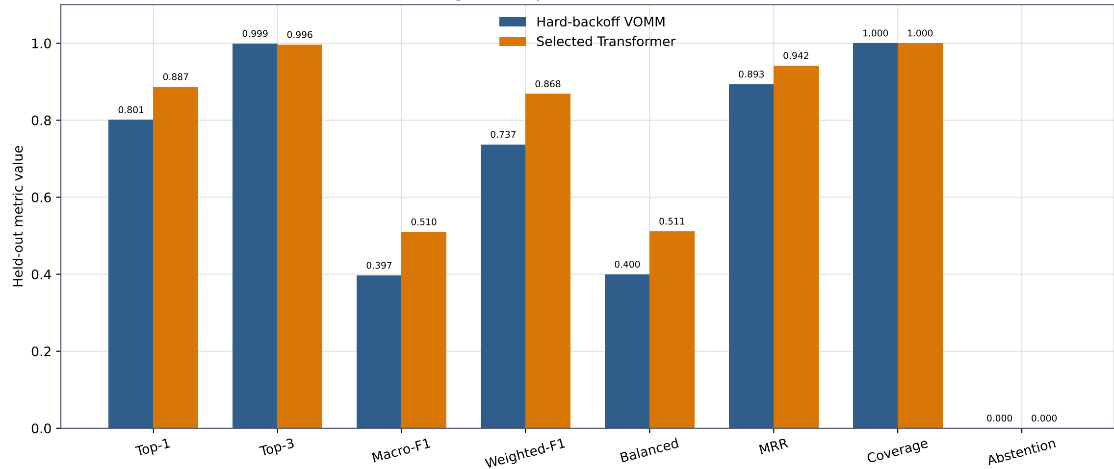
Frozen single-checkpoint Transformer versus VOMM
