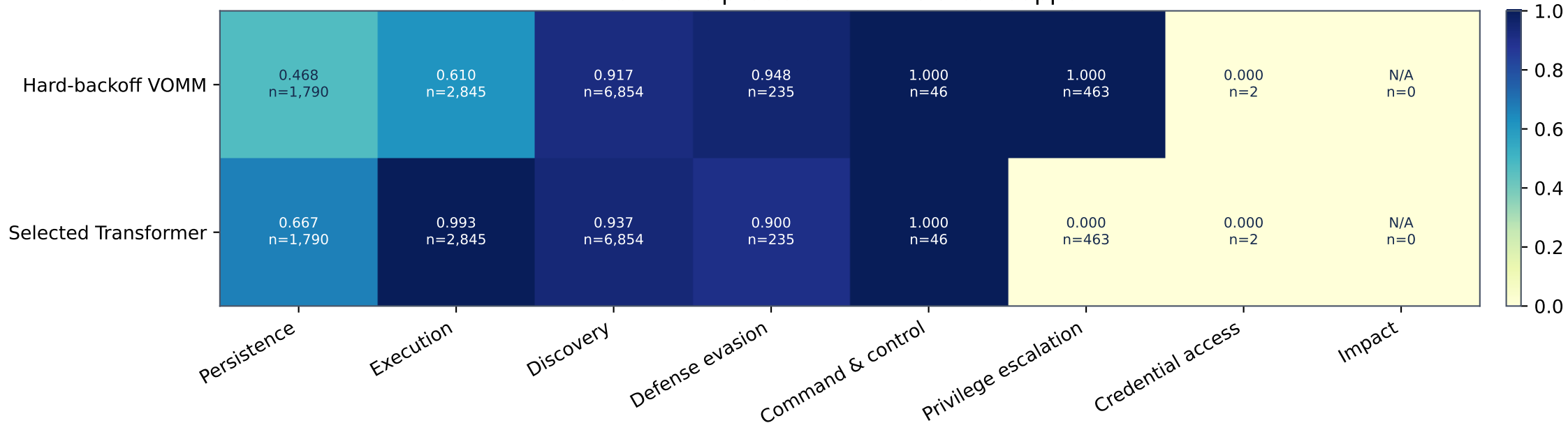
Per-tactic precision with held-out support
