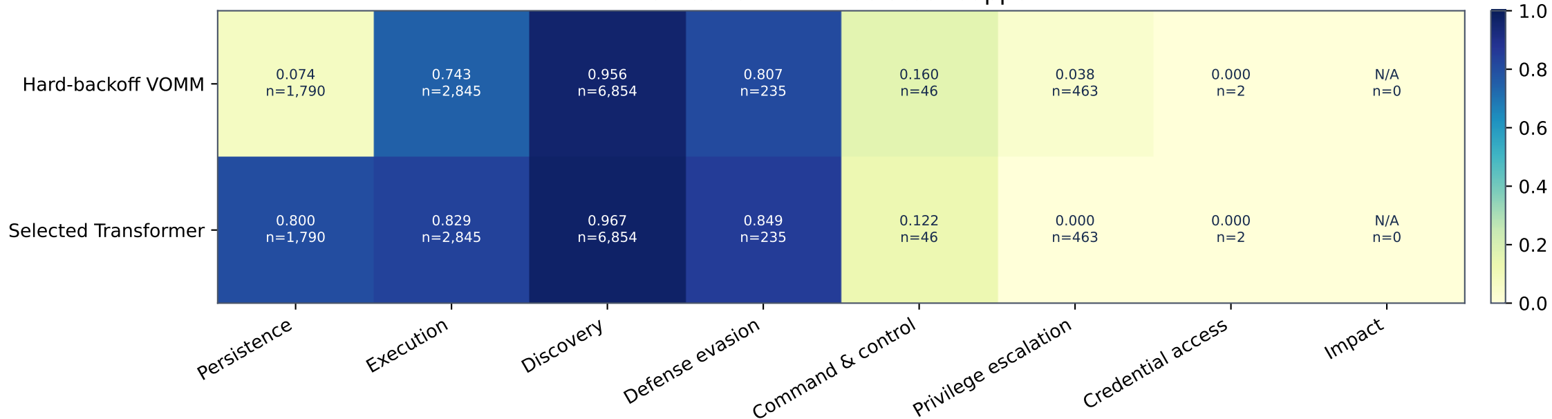
Per-tactic F1 with held-out support
