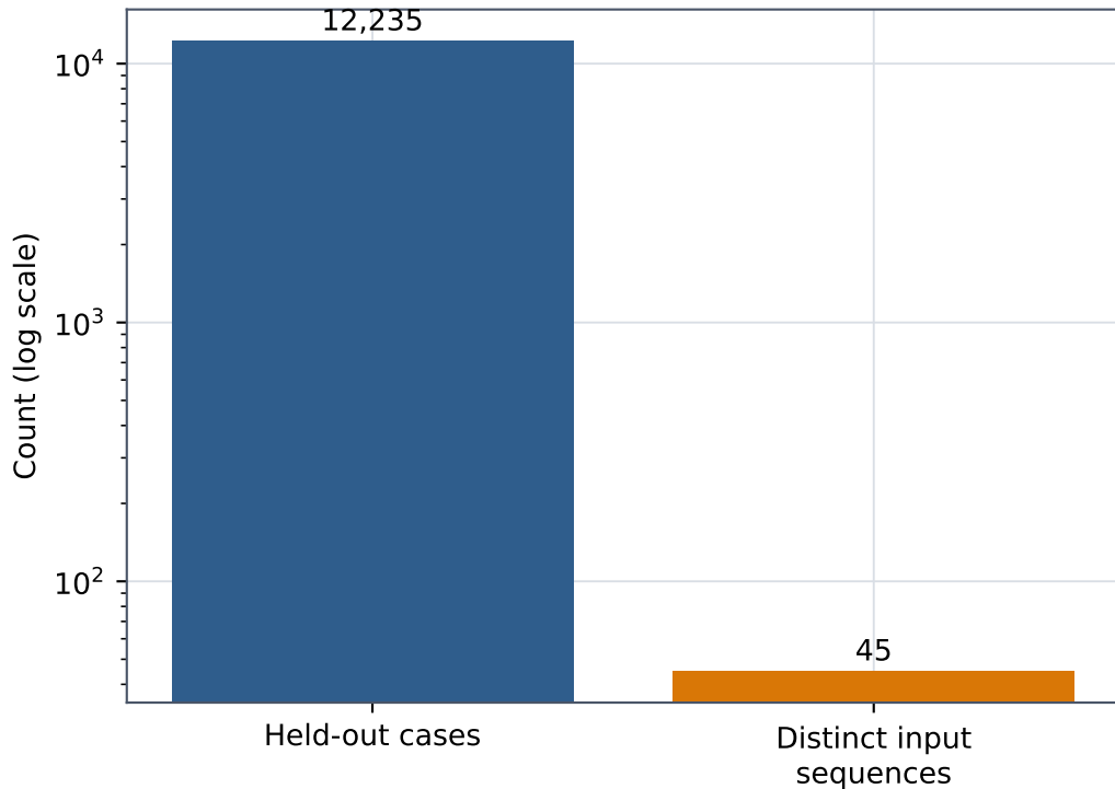
Corpus pattern concentration
