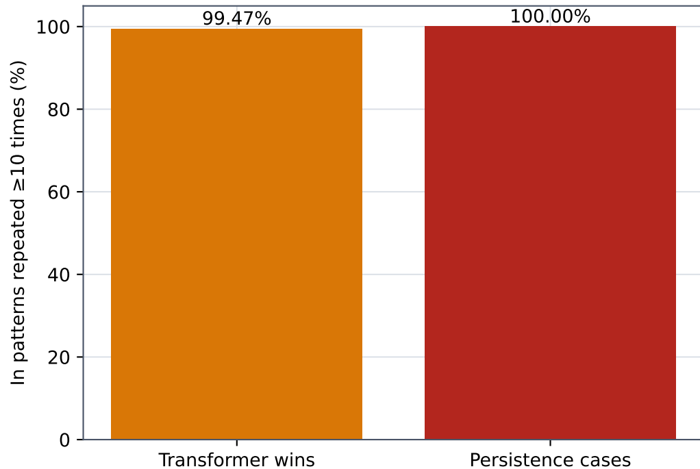
Repeated-pattern exposure
