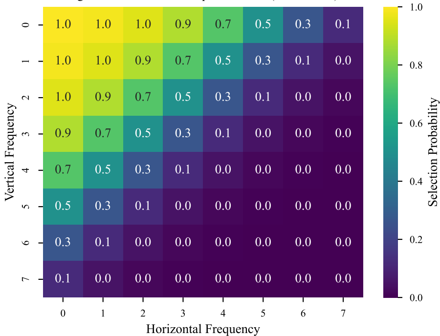
Figure 4: Learned TACS Spectral Mask ( 8 \times 8 DCT)
