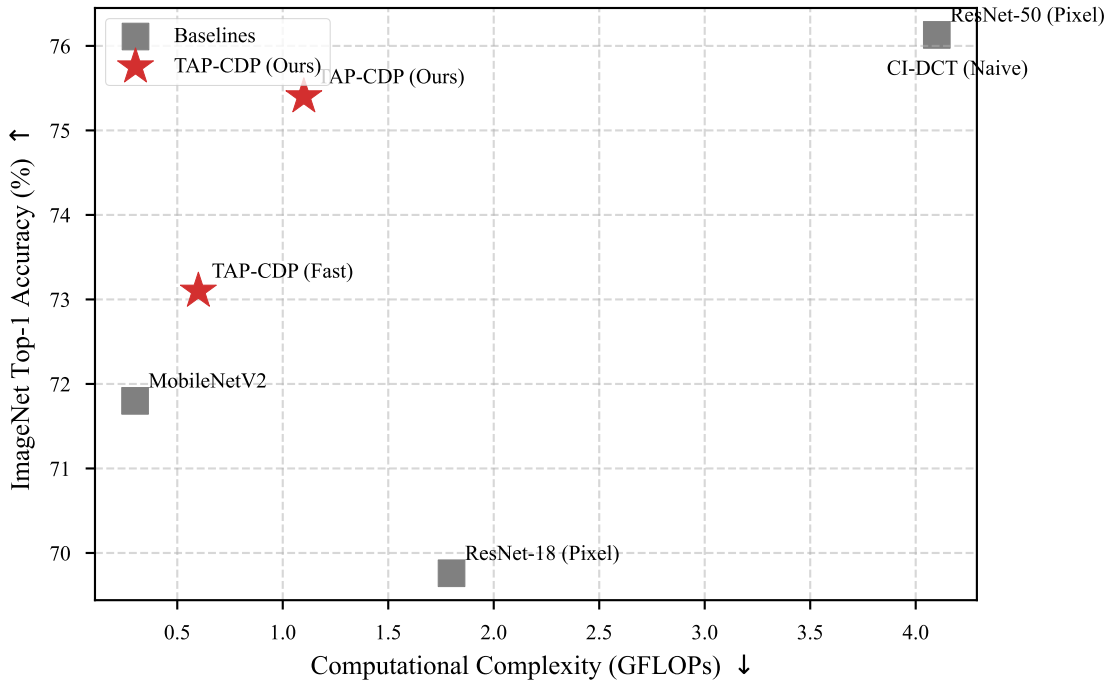
Figure 2: Rate-Accuracy-Complexity Pareto Frontier
