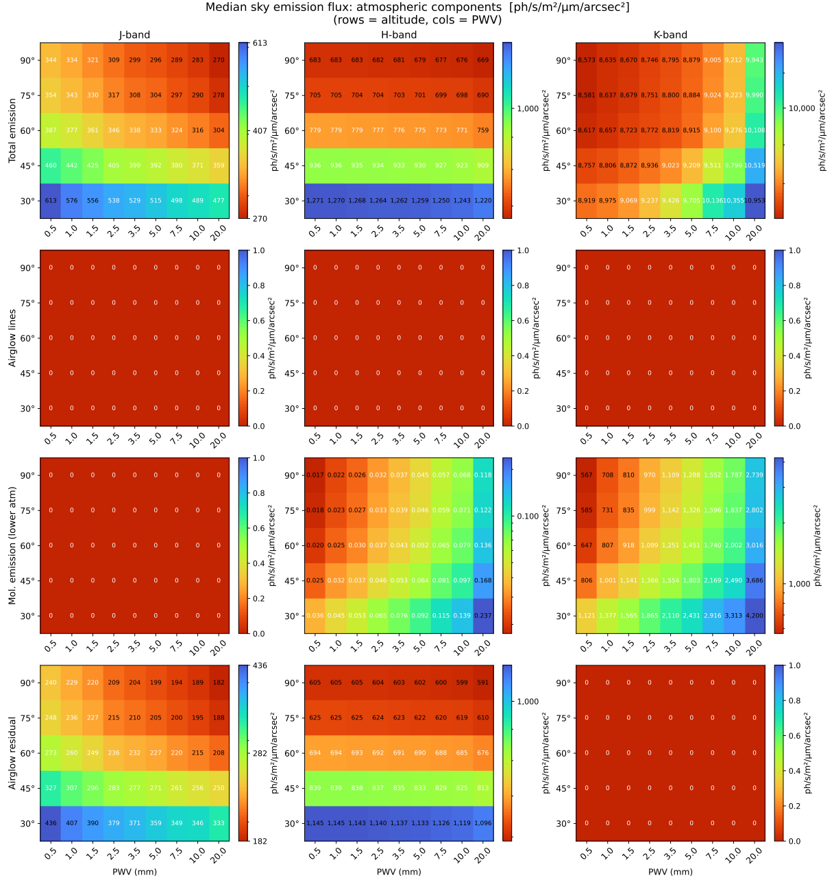
Figure A4: Median sky emission flux for atmospheric emission components (total, airglow lines, molecular emission, airglow residual) across the 5 × 9 grid.
