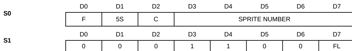
FIGURE 2-2 - STATUS REGISTERS
