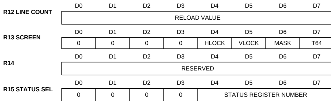
FIGURE 2-1 - EXTENDED REGISTERS (D0 = MSB)
