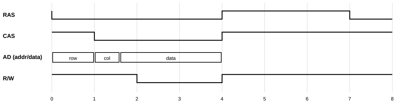
FIGURE 3-3 - WRITE CYCLE
