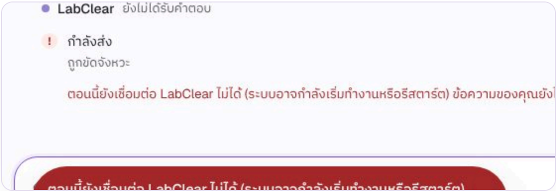
A proxy 502 becomes a Thai message; the text returns to the composer (browser suite 10/10)
