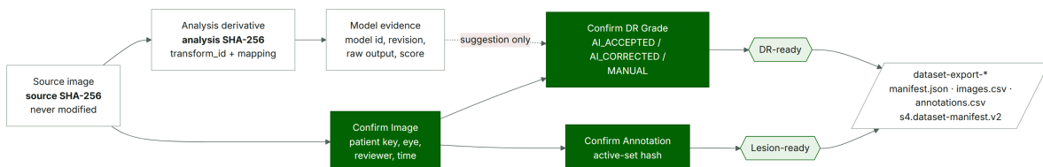
Figure 9.1: Dataset readiness and provenance. Source: docs/adr/architecture/06-dataset-provenance-flow.mmd .
