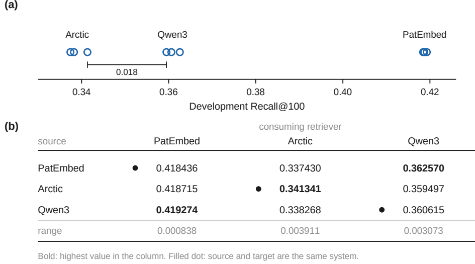
Figure 2: Best construction, for whom? Development Recall@100 for three construction sources and three consuming retrievers. The nominal best source changes with the target, but the spread within a target stays below 0.004 while the bands between targets are separated by substantially more. Development evidence; no single cell carries confirmatory weight.
