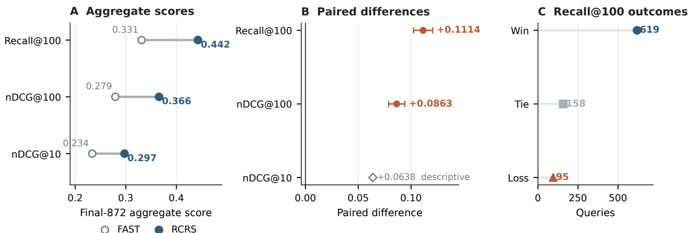
Figure 3: Final-872 comparison of two frozen systems. (A) Aggregate effectiveness. (B) Paired query-level differences and 95% bootstrap confidence intervals; nDCG@10 is descriptive. (C) Query-level Recall@100 wins, ties, and losses.
