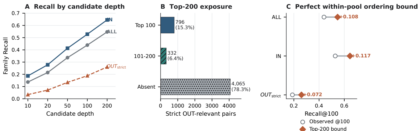
Figure 4: Diagnosis of the unchanged selected RCRS configuration after confirmation. (A) Family-level recall by candidate depth. (B) Pair-level exposure of 5,193 OUT_strict -relevant pairs. (C) Observed Recall@100 and the analytical bound from perfect ordering of the frozen Top-200 pool. IN and OUT are relation-scoped and may overlap by query.
