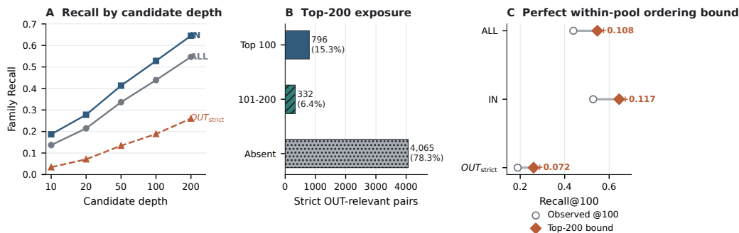
Figure 4: Diagnosis of the unchanged selected RCRS configuration after confirmation. (A) Family-level recall by candidate depth. (B) Pair-level exposure of 5,193 OUT_{strict} -relevant pairs. (C) Observed Recall@100 and the analytical bound from perfect ordering of the frozen Top-200 pool. IN and OUT are relation-scoped and may overlap by query.
