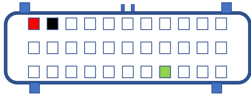
33 Pin
