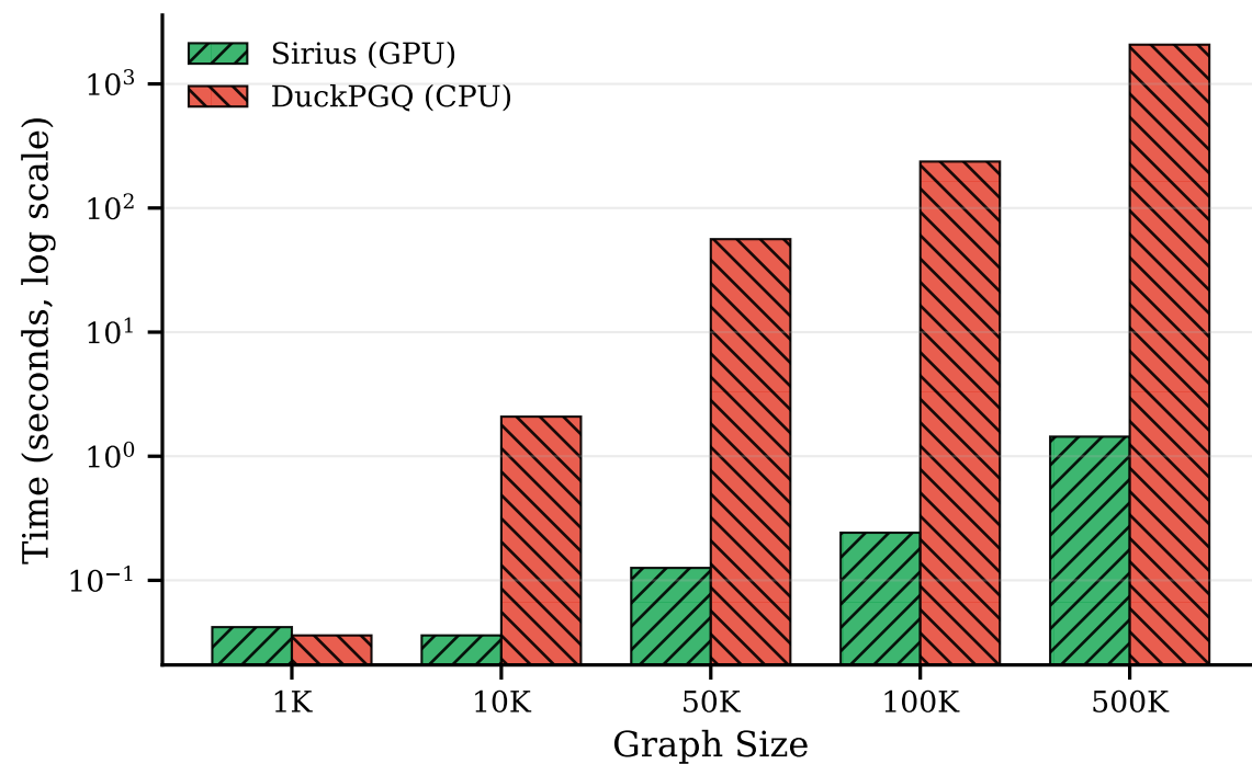
Shortest Path (Unweighted)
