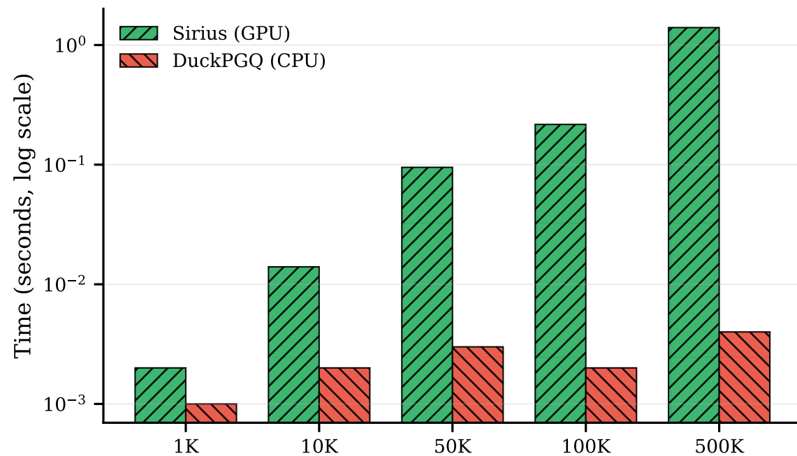
Shortest Path (Unweighted)
