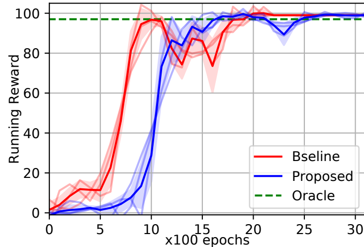
Comparison of average runs
