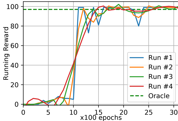
Proposed: Meta-DNN
