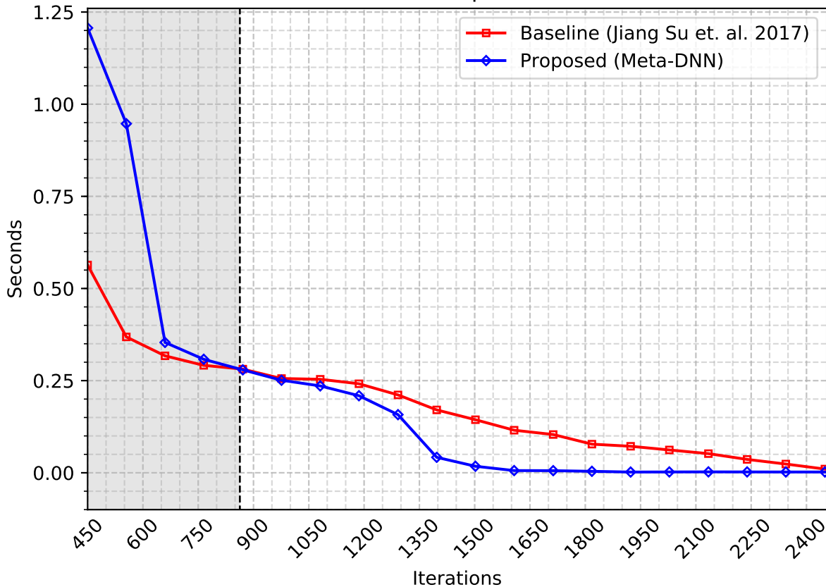
Wall clock time per inference
